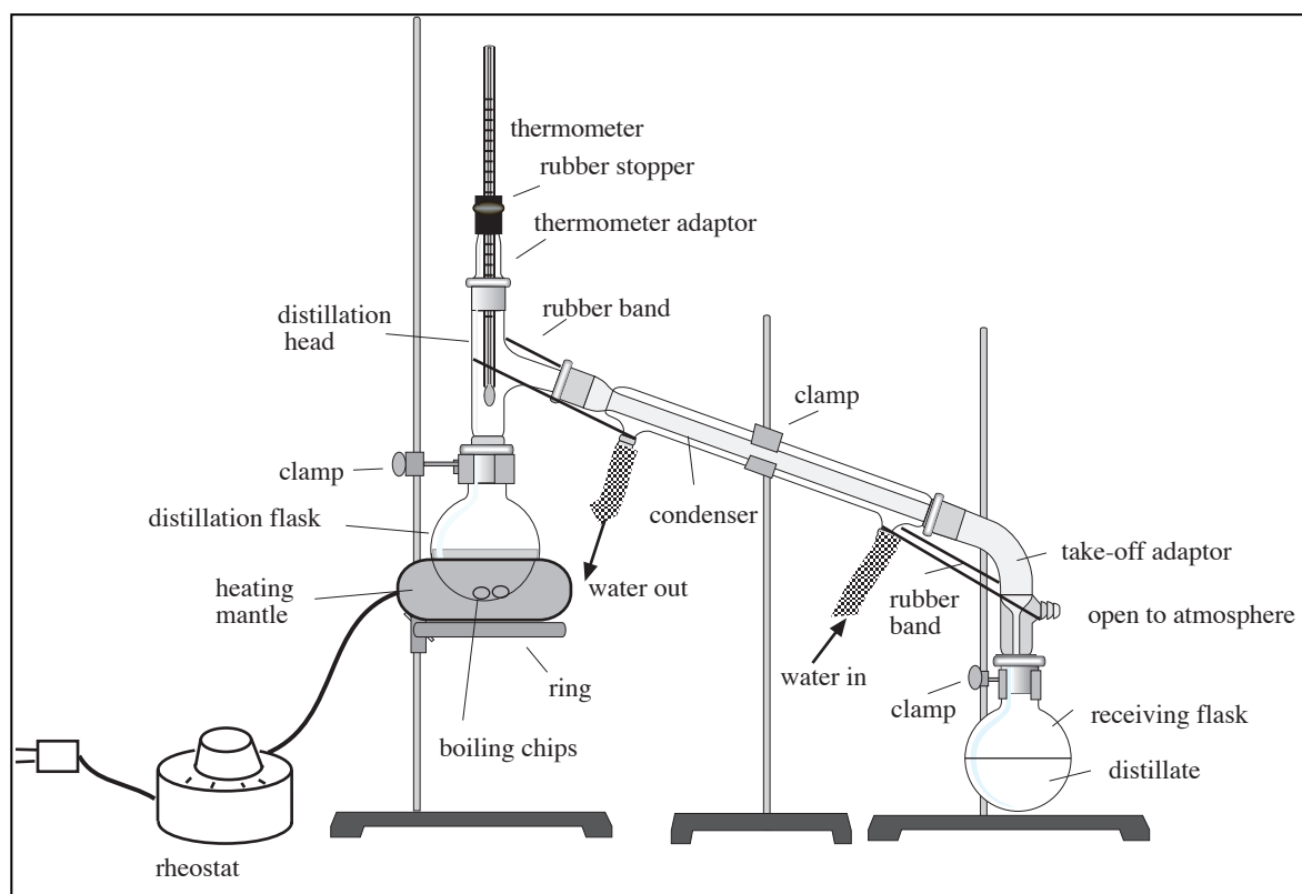
Figure 2. A simple distillation apparatus used for steam distillation. Sketch this diagram into the procedure portion of your notebook.
