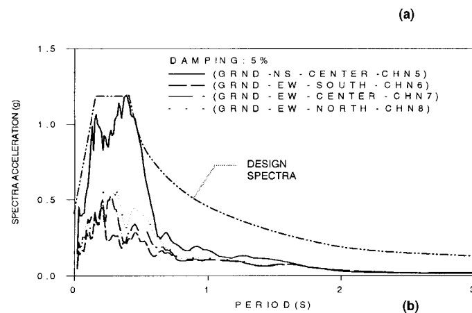
FIG. 2. (a) Recorded Ground Acceleration Time Histories during Northridge Earthquake; (b) Acceleration Response Spectra at Ground/Foundation Level
