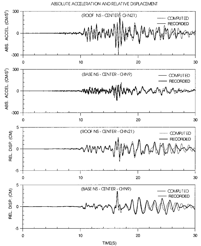
FIG. 5. Comparison of Recorded and Computed Response in Northridge Earthquake in NS Direction (Note: Relative Displacement at Roof Is with Respect to Base and Base Is with Respect to Ground)
